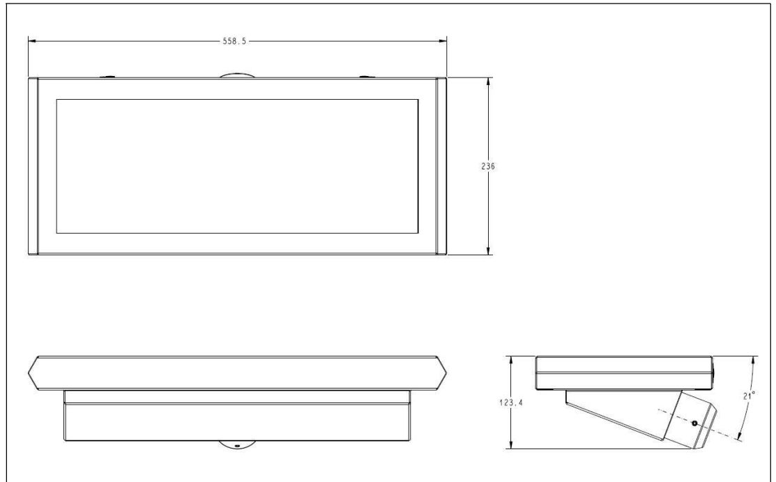
Figure 3.5 Standard housing with option F-R, prepared for pipe mounting
